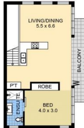
GRANNY FLAT (CARPORT UNDER)
